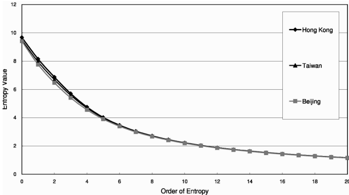
Fig. 3. Higher order average joint character entropy of Chinese.
