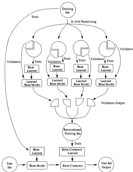
Fig. 1. Piped architecture with n-fold partitioning.
