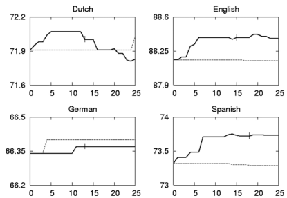
Fig. 2. Performance improvement is not reliably obtained without n-fold partitioning. (x-axis = number of rules learned, y-axis = F-Measure; bold = NTPC, dashed = without n-fold partitioning).
