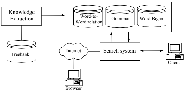
Fig. 2. The Tree-Searching system
