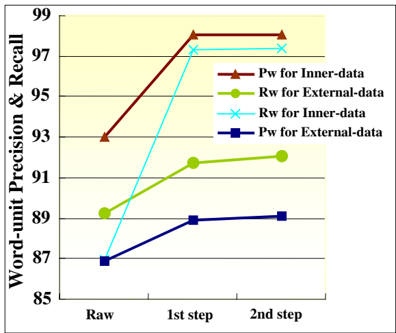
Fig. 1. Performance Change According to Training-data Edition
