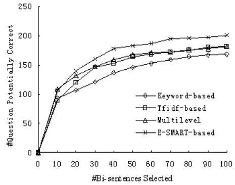
Fig. 4. Sentence Retrieval Comparison
