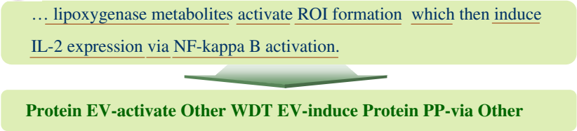
Fig. 2. An example of sentence normalization.
