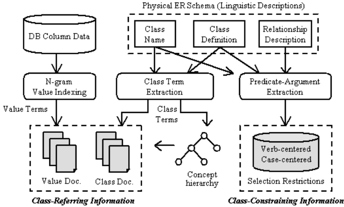
Fig. 1. Translation Knowledge Construction
