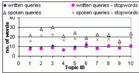
Fig. 5. Avg length of queries across topics.
