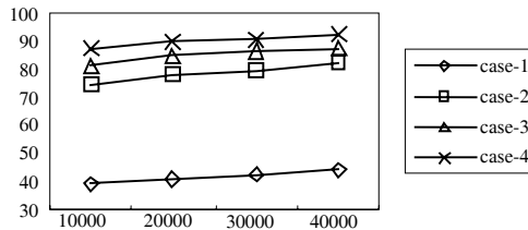
Fig. 3. Coverage rates vs. size of treebanks
