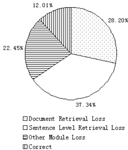
Fig. 2. Loss Distribution
