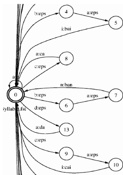
Fig. 4. Part of the FST for pinyin syllabification
