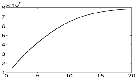
Fig. 5. Treelet numbers
