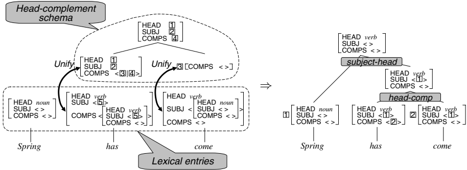
Fig. 3. HPSG parsing.
