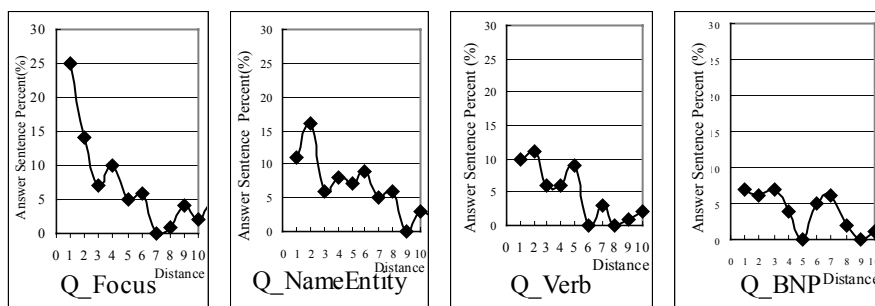
Fig. 2. Distribution of Q_Tag Around Answer
