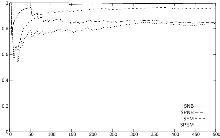
Fig. 1. Legitimate recall achieved by four learning strategies on the SpamAssassin corpus with 40% spam, accumulated over the number of messages received.
