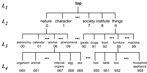
Fig. 2. Concept hierarchy of the Kadokawa thesaurus
