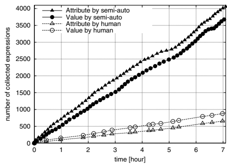
Fig. 4. Number of collected expressions (car).
