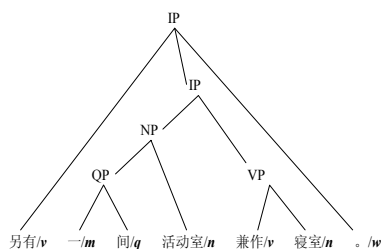
Fig. 1. Word level parsing tree
