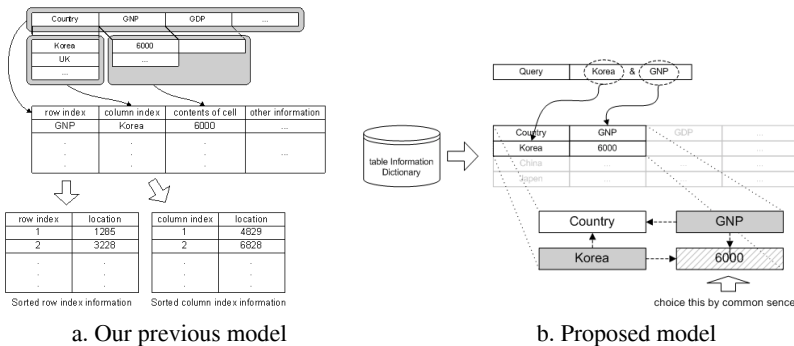
Fig. 5. Model of Information Extraction
