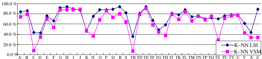
Fig. 2. The macro-averaged F 1 curves for each category using k-NN VSM versus k-NN LSI
