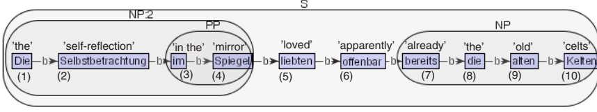
Fig. 3. Phrase structure represented as hierarchical graph.
