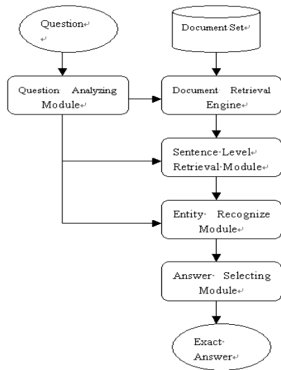
Fig. 1. The Architecture of QA system
