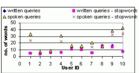
Fig. 6. Avg length of queries per user.
