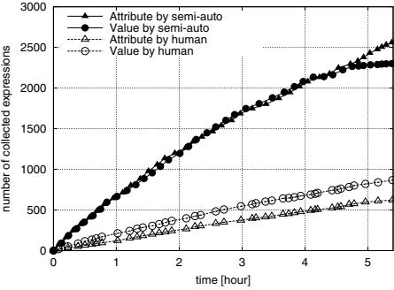
Fig. 5. Number of collected expressions(game).
