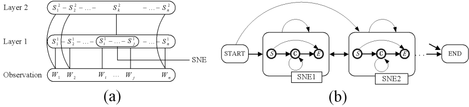
Fig. 1. Cascaded models (a) vs. hierarchical models (b). SNE means simple named entity predicted at the lower level.
