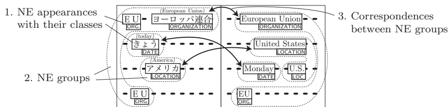
Fig. 1. Representation of NE Translations in a Document Pair.
