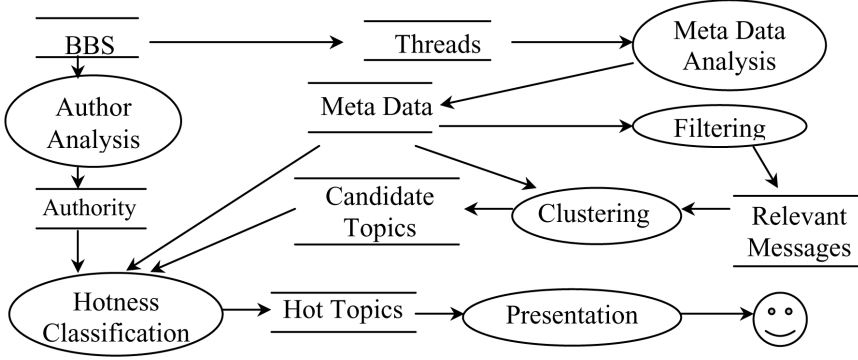
Fig. 1. Architecture of hot topic retrieval
