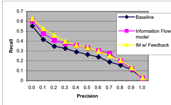
Fig. 2. Precision-recall curves comparing the baseline model with information flow models
