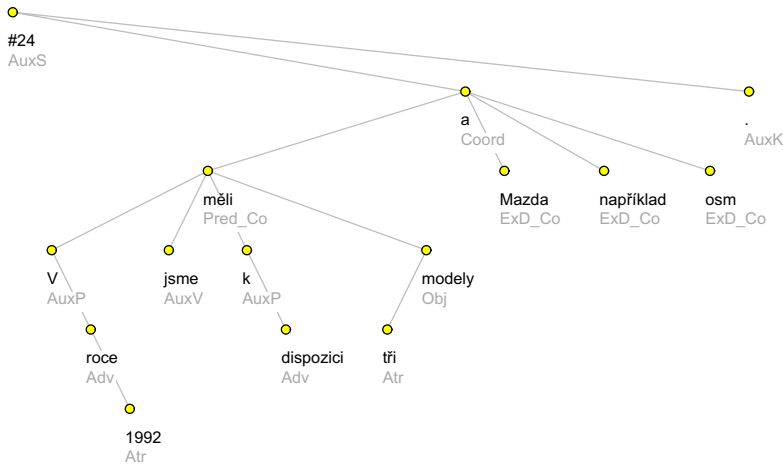
Fig. 3. Analytical annotation of the sentence “ V roce 1992 jsme měli k dispozici tři modely a Mazda například osm. ” [In the year 1992 we had at our disposal three models and Mazda (had) for example eight (models).]
