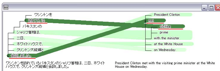
Fig. 1. Annotation Tool.
