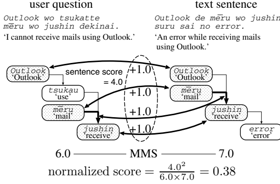
Fig. 4. Score calculation.
