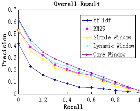
Fig. 4. Overall Accuracy
