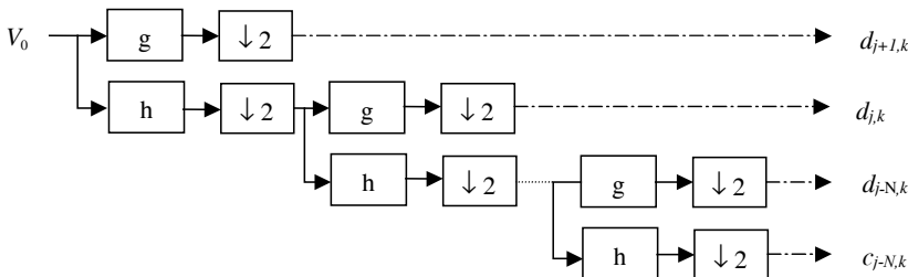
Fig. 1. Two-band analysis tree for a discrete wavelet transform
